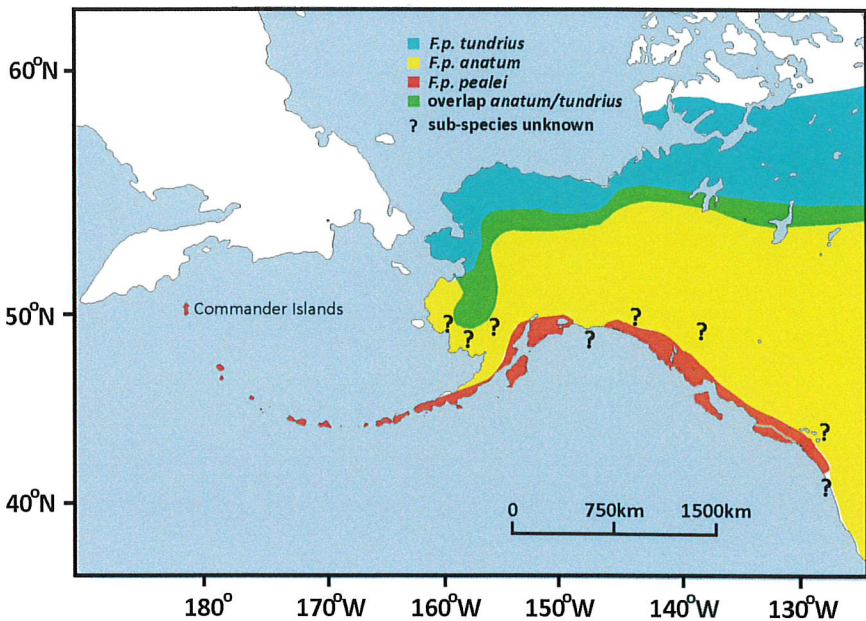
Figure 2.14 Distribution of the three North American Peregrine sub-species in Alaska and neighbouring north-west Canada. Redrawn from Talbot (2017). Note that the map is a flattened 3D projection resulting in the spacing of the lines of latitude appearing unequal.
